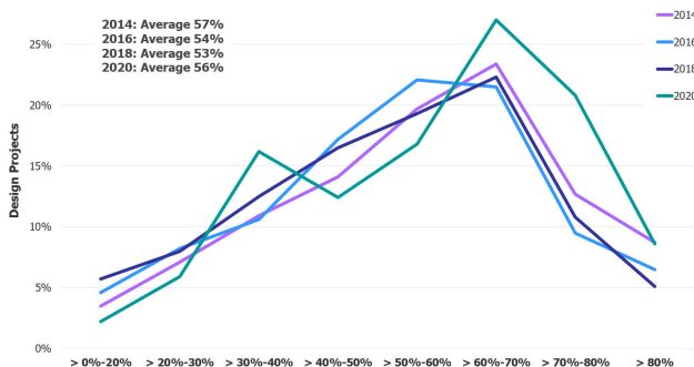
Fig. 7: Percentage of IC/ASIC project time spent in verification.
