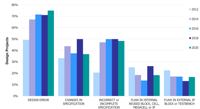
Fig. 5: Root cause of functional flaws.
