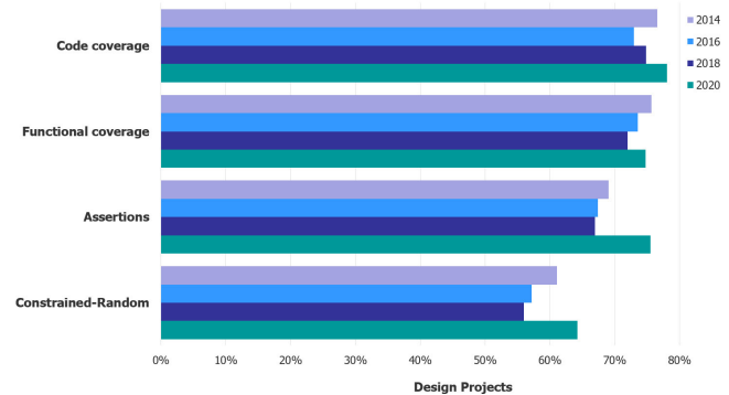
Fig. 20: IC/ASIC project simulation technique trends.
