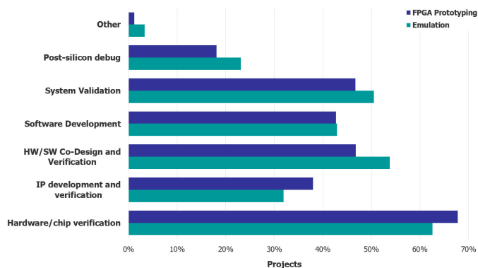
Fig. 21: Why was emulation or FPGA prototyping used?
