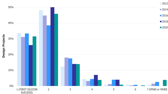
Fig. 3: IC/ASIC spins required before production.
