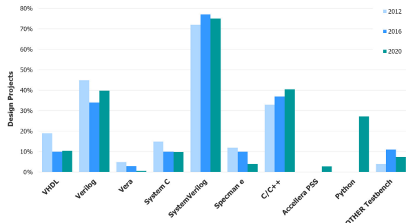
Fig. 16: IC/ASIC project verification language adoption.
