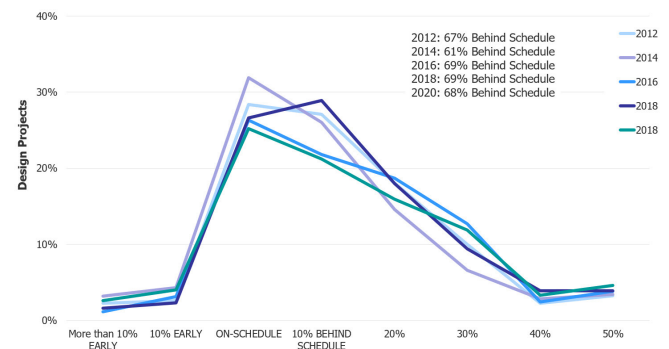
Fig. 6: Actual IC/ASIC project completion compared to original schedule.
