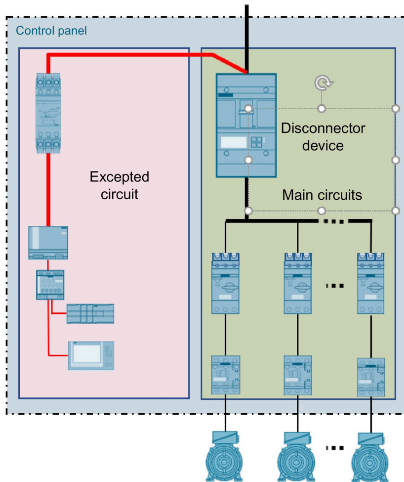
Figure 5-11 Example of the configuration of an excepted circuit
