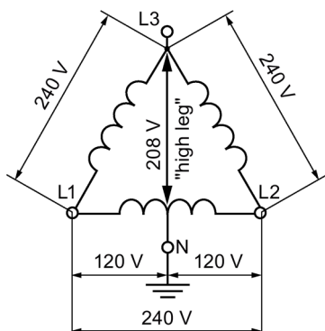
Figure 5-6 Midpoint grounded delta 240/10 V 3-phase 4 wire
