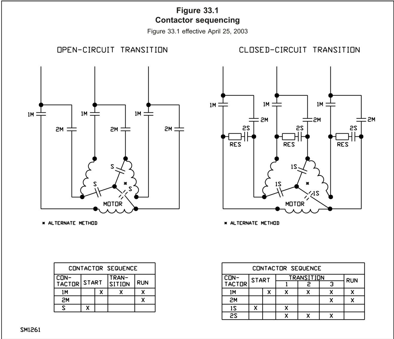
Figure 6-26 Wye-delta circuits in accordance with UL 508A (source: UL 508A, Figure 33.1)
