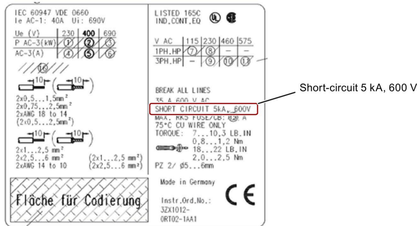
Figure 6-36 Example of 3RT contactor label
