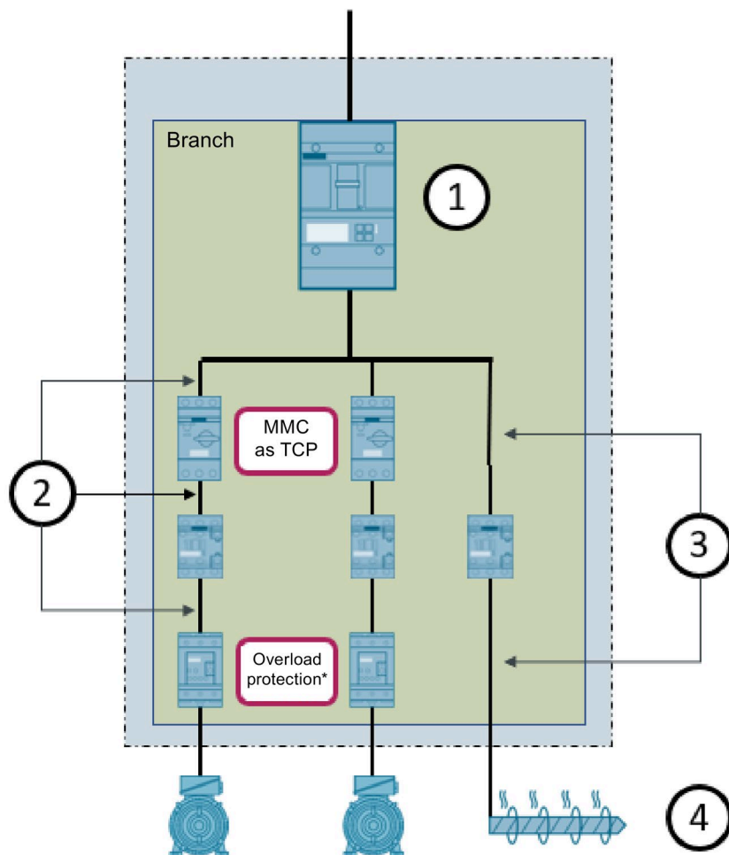
Figure 6-32 Group installation method 3
