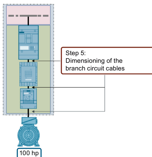
Figure 6-11 Sizing of the wiring
