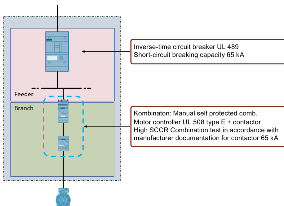
Figure 6-40 Example of "Determining the SCCR on the basis of tested device combinations"
