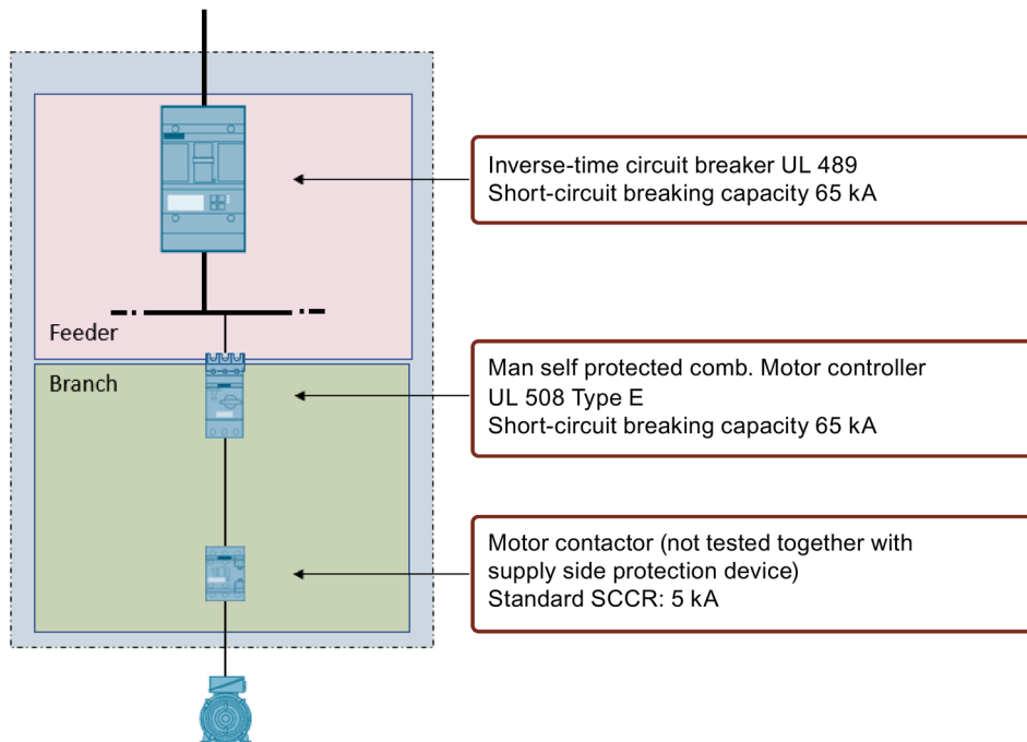
Figure 6-37 Example of "Determining the SCCR on the basis of the device marking"
