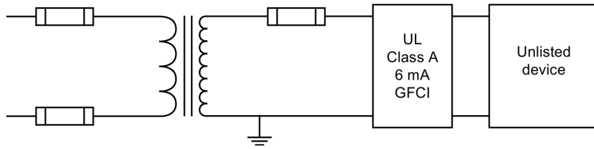
Figure 7-9 Design of a control circuit for an unlisted component
