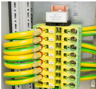
Figure 13-7 Siemens 8WH grounding terminals
