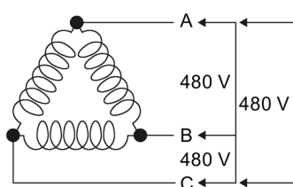
Figure 5-5 Grounded delta system, 480 V, 3-phase, 3-wire
