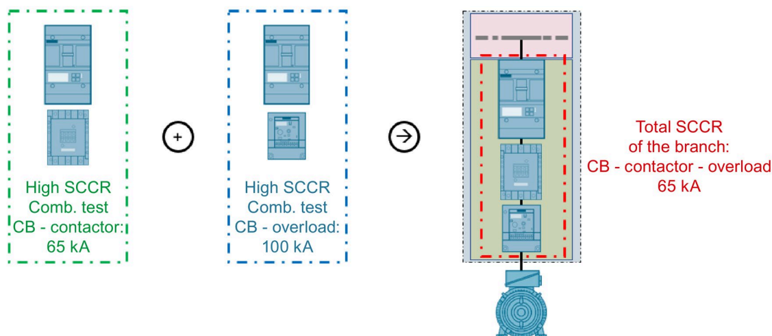
Figure 6-14 Combined SCCR of all components in the feeder
