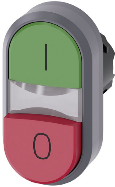
Figure 13-25 Siemens twin pushbutton with 3SB31 00 indicator light function identification on the actuator
