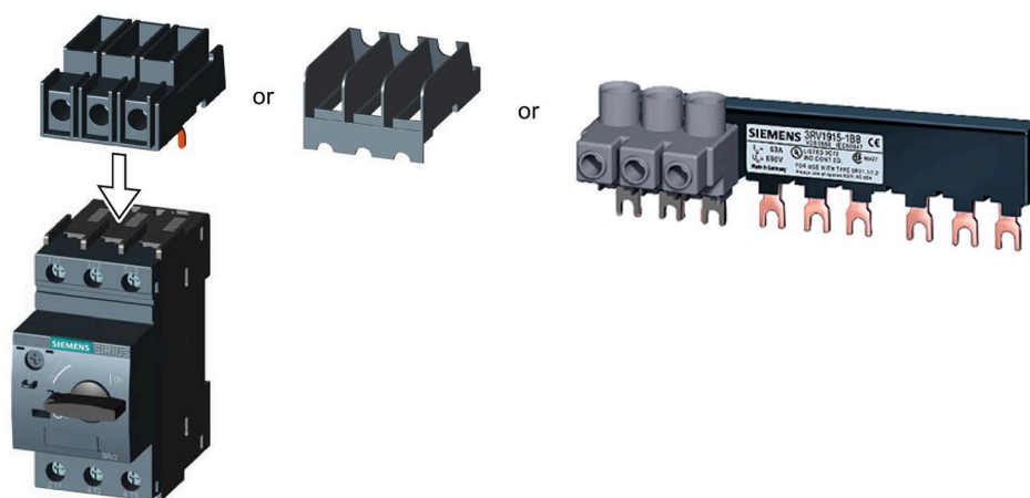
Figure 5-2 Example of "Manual self-protected combination motor controller" according to UL 508 Type E
