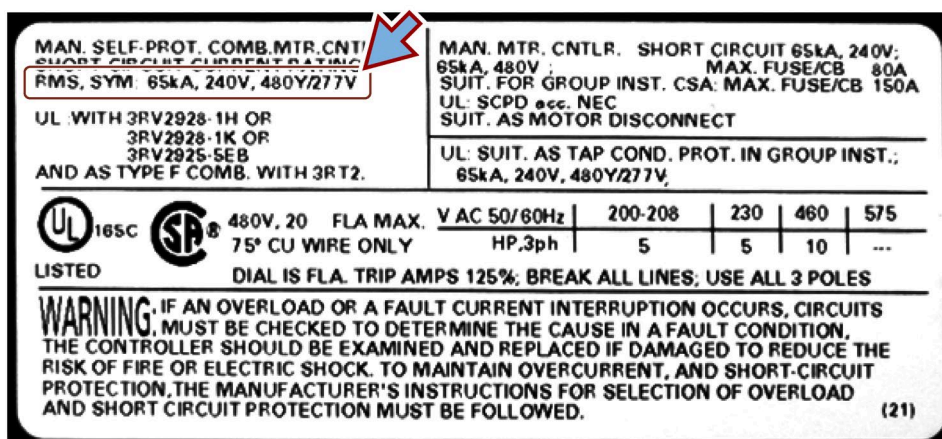
Figure 5-7 Sample nameplate of a motor circuit breaker approved for 65 kA at 240 V and 480Y / 277 V
