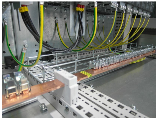
Figure 8-1 Grounding concept of an industrial control panel
