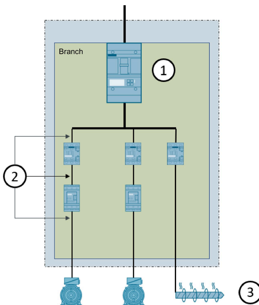
Figure 6-30 Group installation without tap conductor protection method 2
