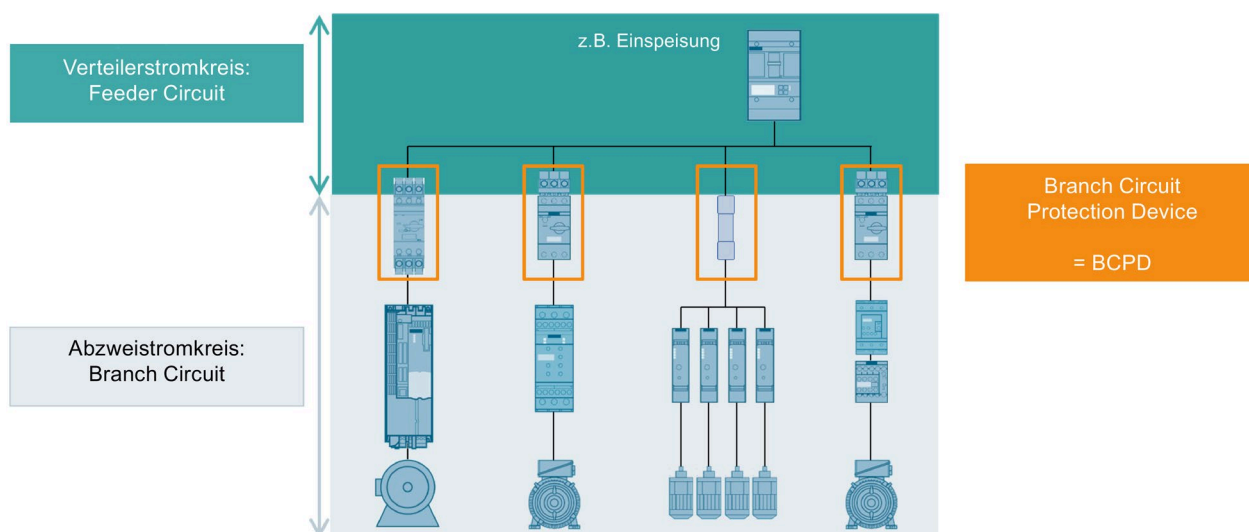
Figure 5-1 Illustration Feeder Circuit – Branch Circuit
