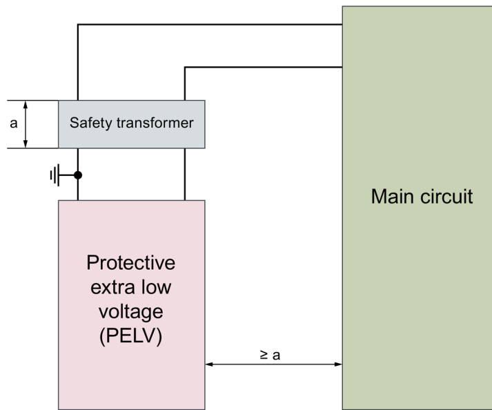
Figure 5-25 Example configuration of a protective extra low voltage (PELV) circuit
