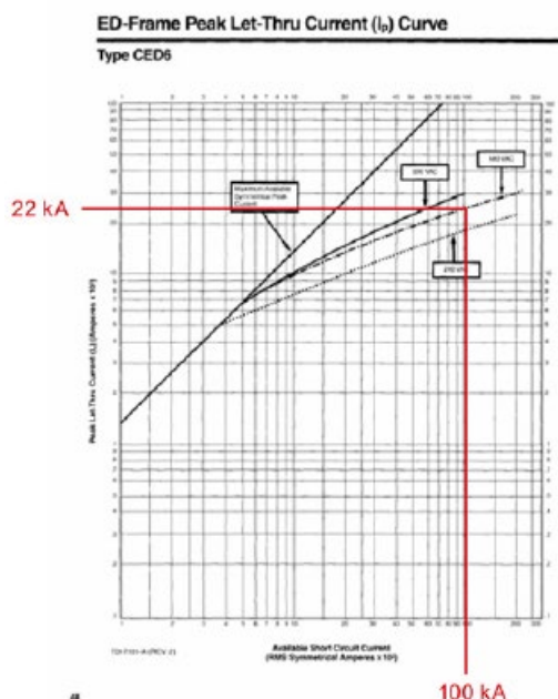
Figure 6-42 Let-through characteristic of a circuit breaker marked as "current limiting"
