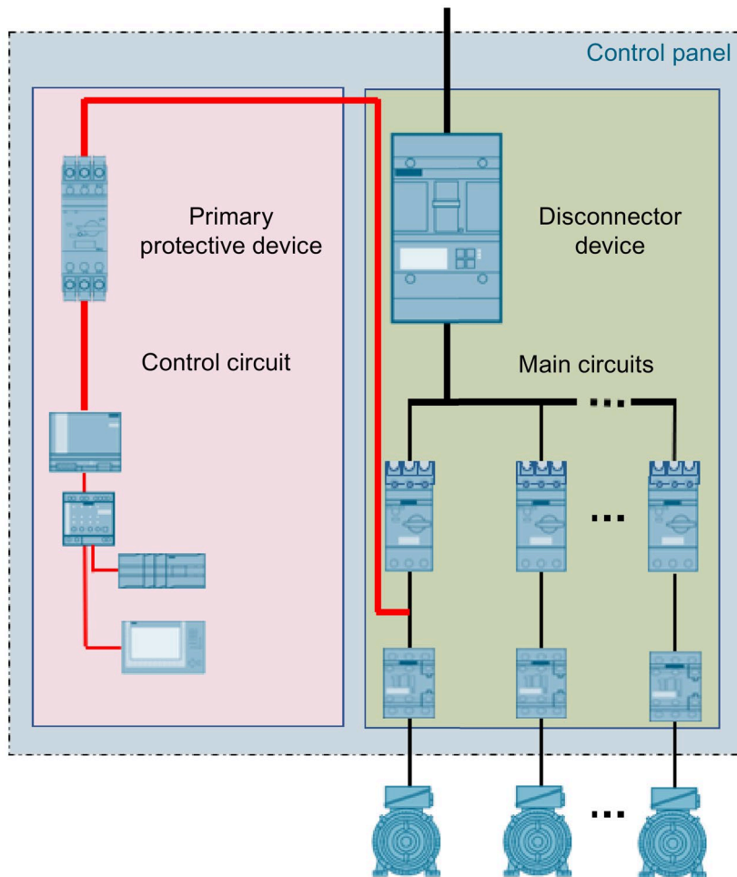
Figure 7-4 Control circuit tapped downstream of the "Branch Circuit Protective Device"
