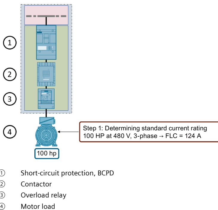
Figure 6-6 Determining the motor standard current
