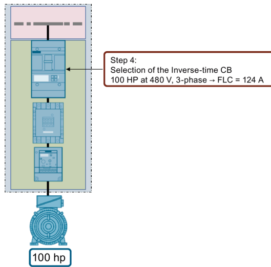
Figure 6-9 Selection of the short-circuit protective device
