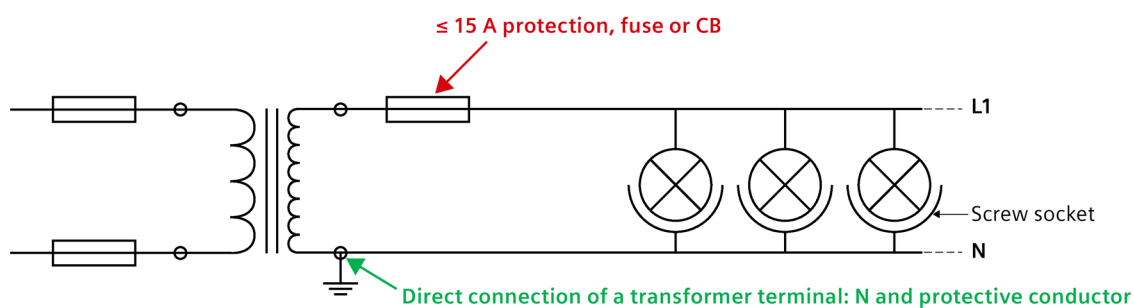
Figure 8-4 Lighting circuits
