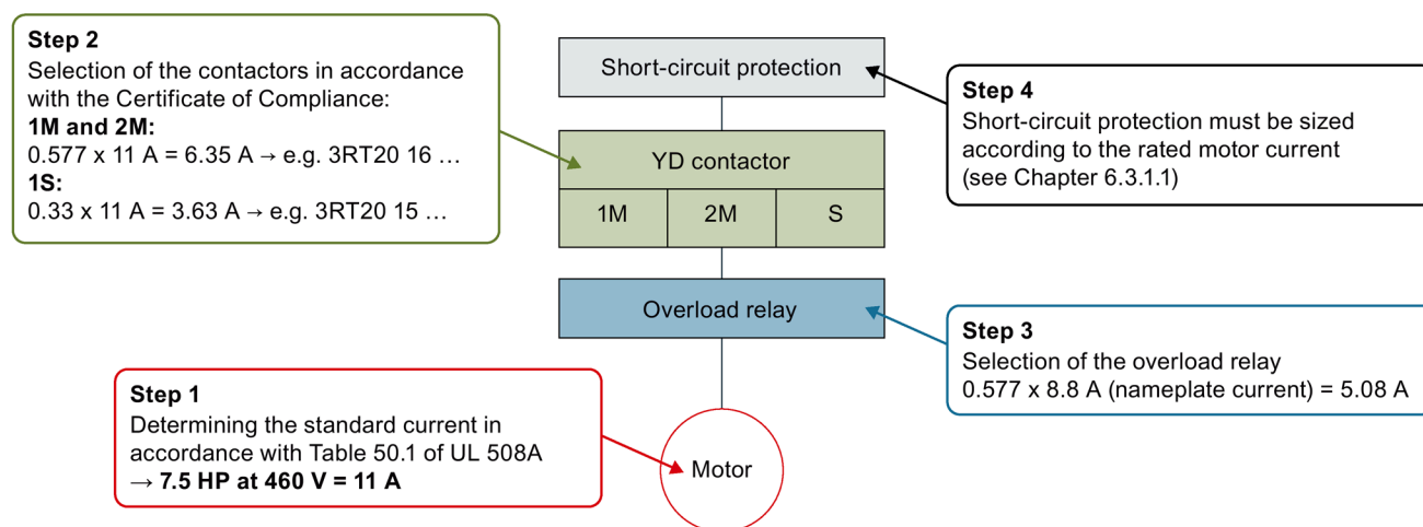
Figure 6-28 Sizing of a contactor assembly for wye-delta start
