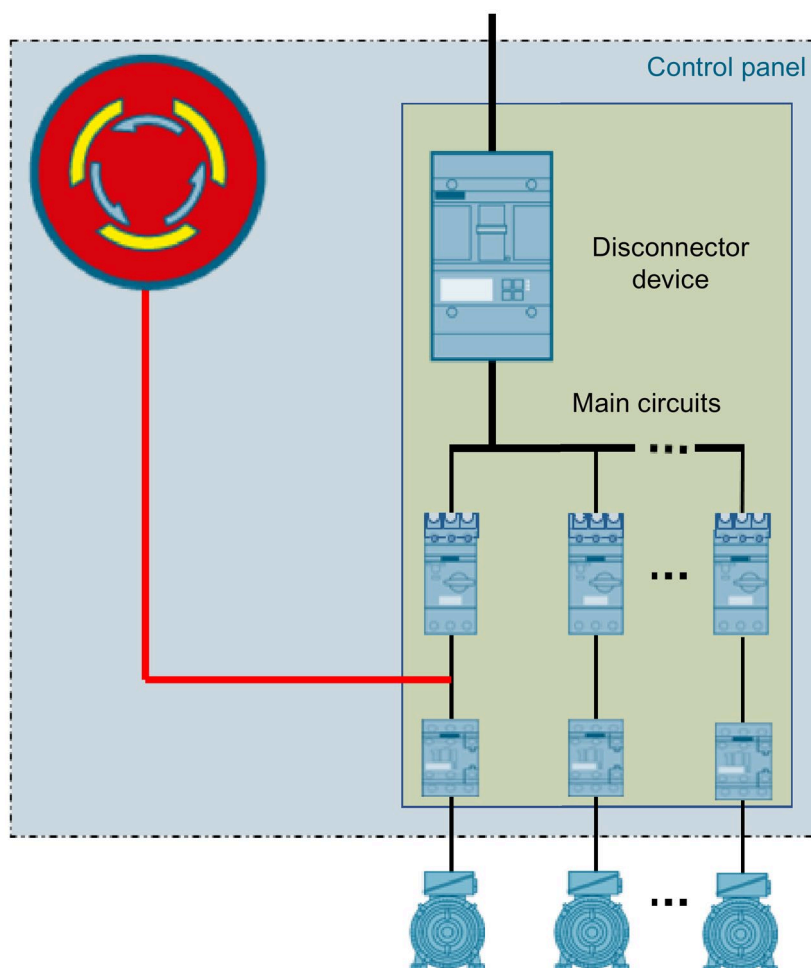
Figure 7-7 Tapping downstream of the main control switch and downstream of the "Branch Circuit Protective Device" of a motor feeder without control circuit components inside the cabinet without remote control
