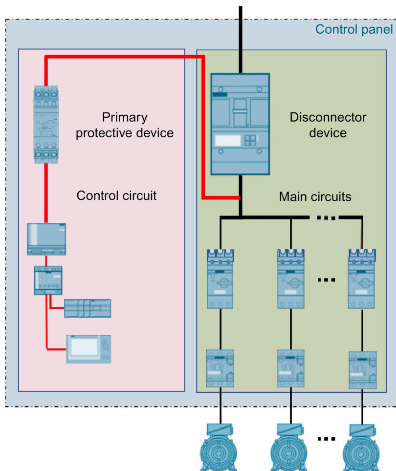
Figure 7-3 Control circuit tapped downstream of the main control switch and upstream of the load branch circuits
