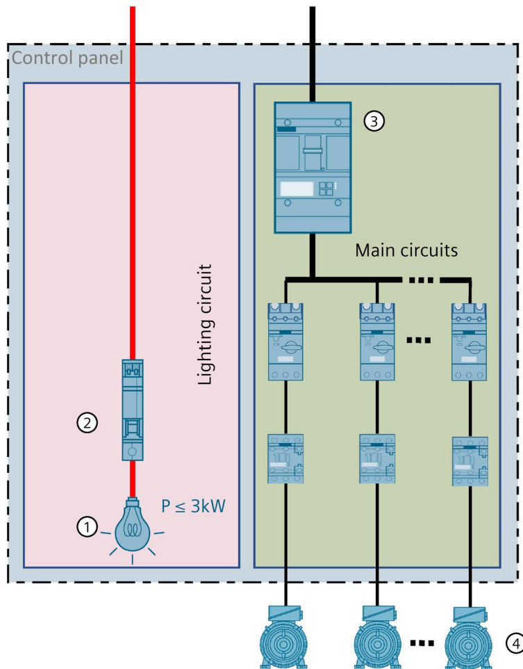
Figure 12-8 Structure machine lighting, using the example inside industrial control panel option 5
