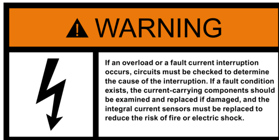
Figure 13-16 Example of warning notice for motor circuit breakers
