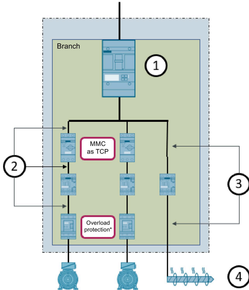
Figure 6-31 Group installation with tap conductor protection method 2
