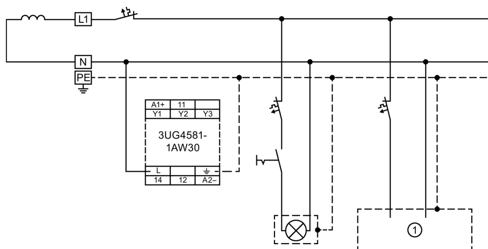
Figure 8-3 Ungrounded control circuits
