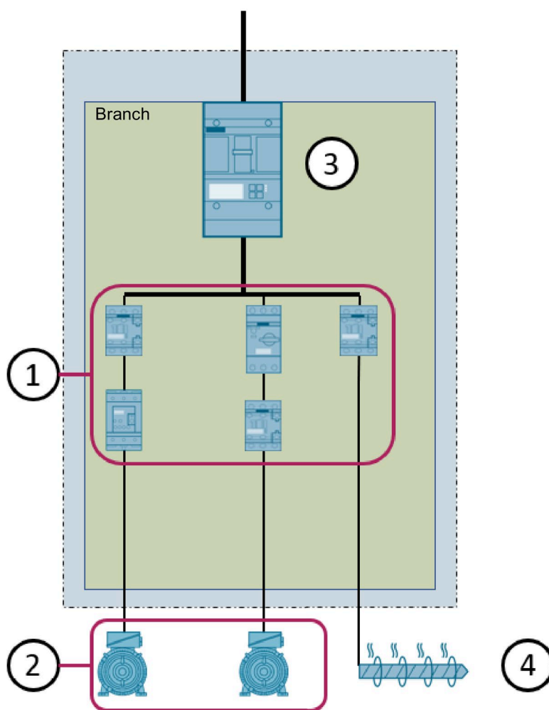
Figure 6-29 Group installation method 1
