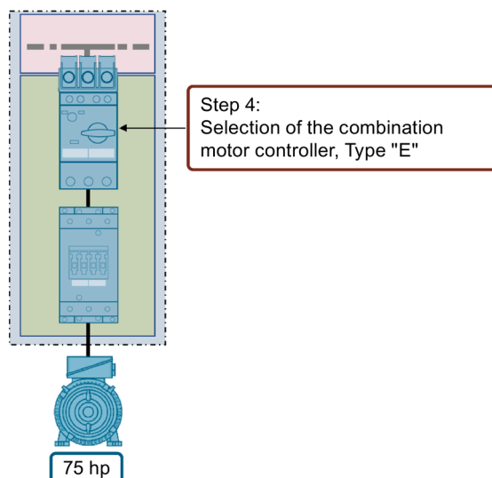
Figure 6-22 Selection of the protection device
