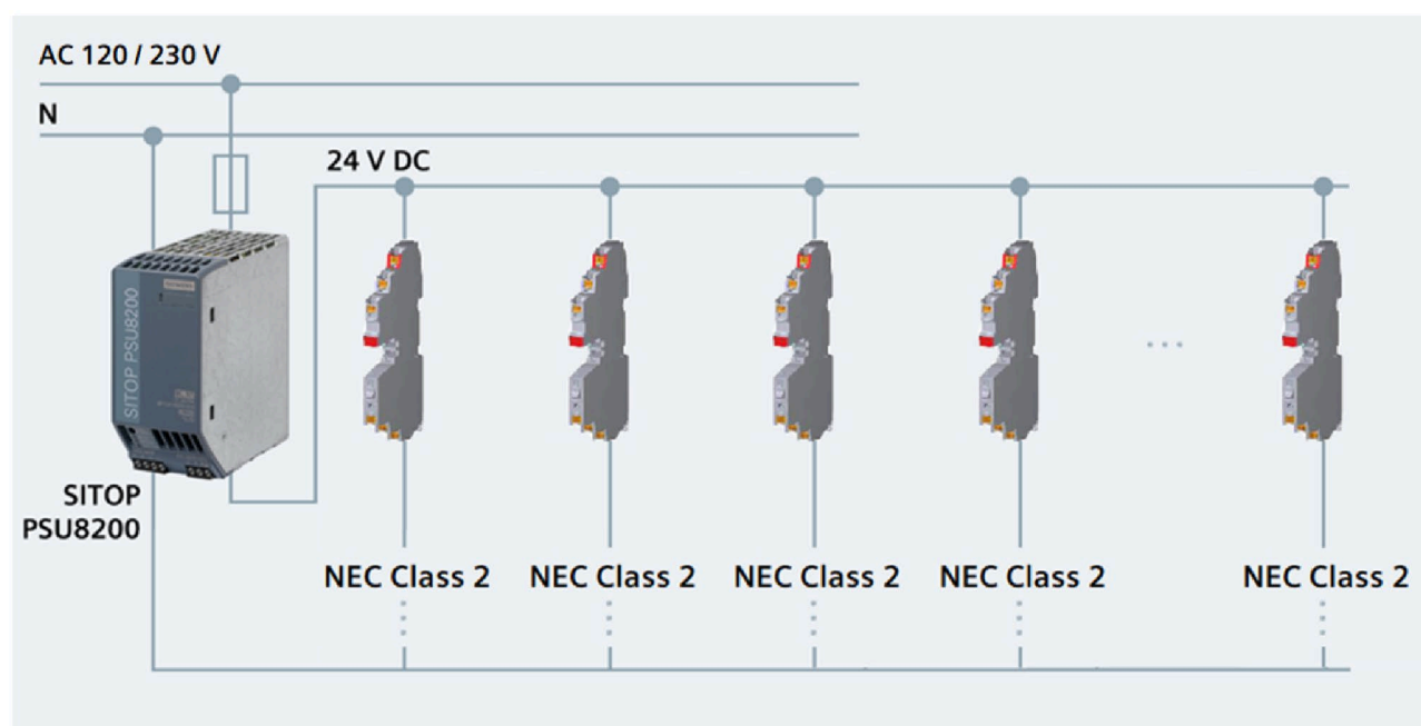
Figure 7-5 Device protection switch 5SK9
