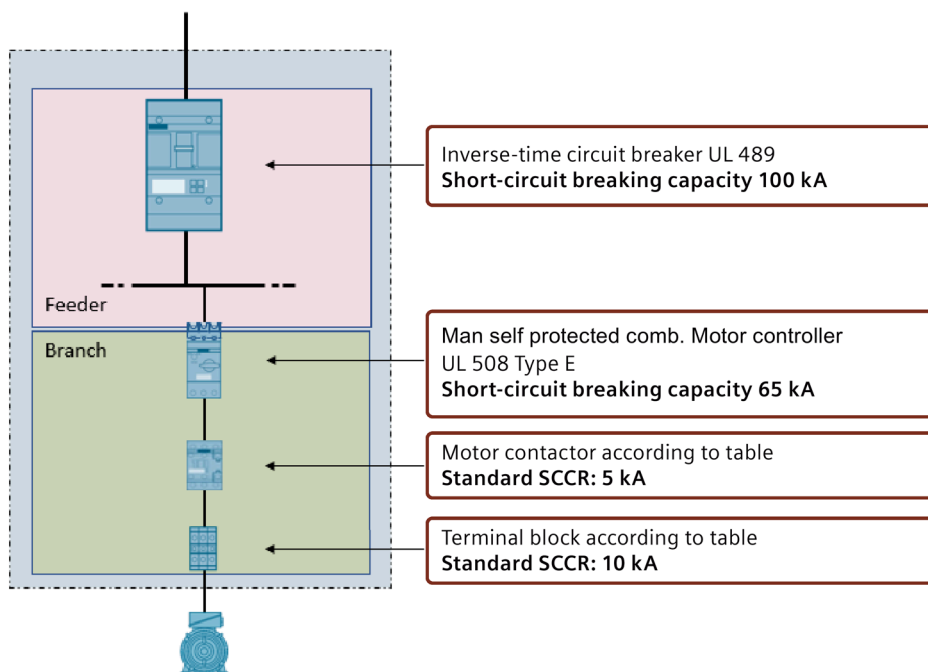
Figure 6-38 Example "Determination of the Combined SCCR of the feeder on the basis of the standard SCCR of the individual components"
