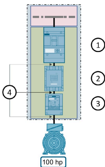
Figure 6-10 Fully dimensioned branch circuit
