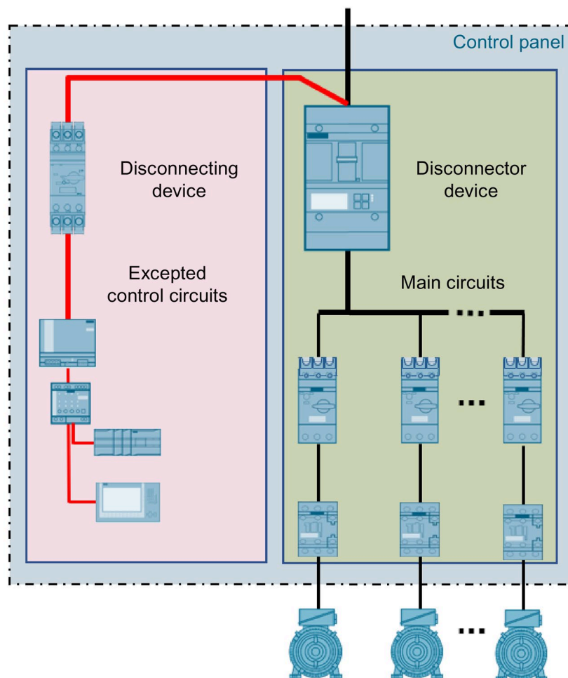
Figure 7-2 Control circuit tapped upstream of the main control switch
