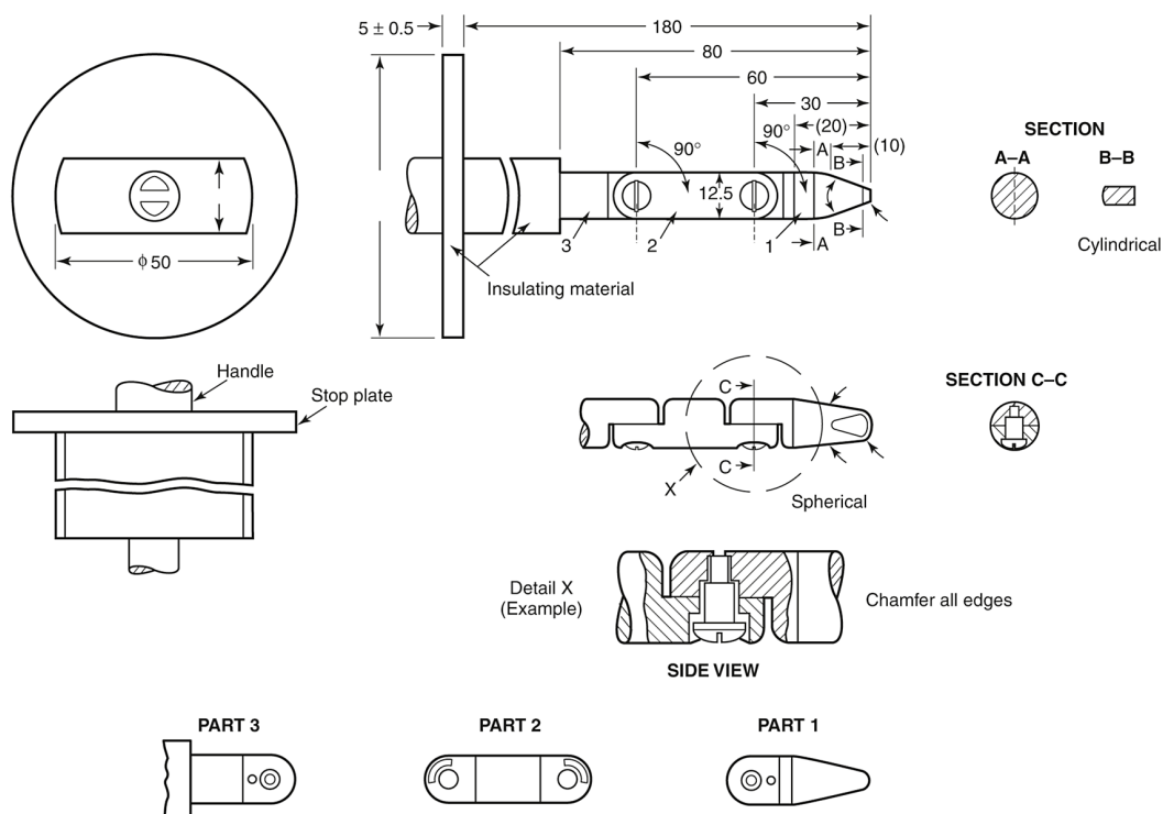
Figure 5-17 Test finger in accordance with NFPA 79, Fig. 6.2.3
