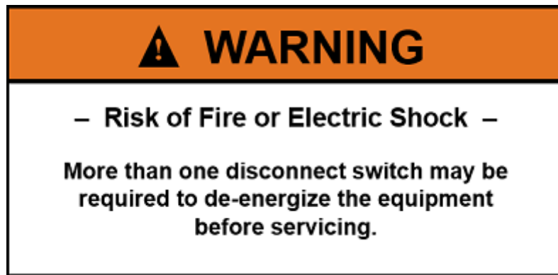
Figure 5-15 Warning label excepted circuit (UL 508A)
