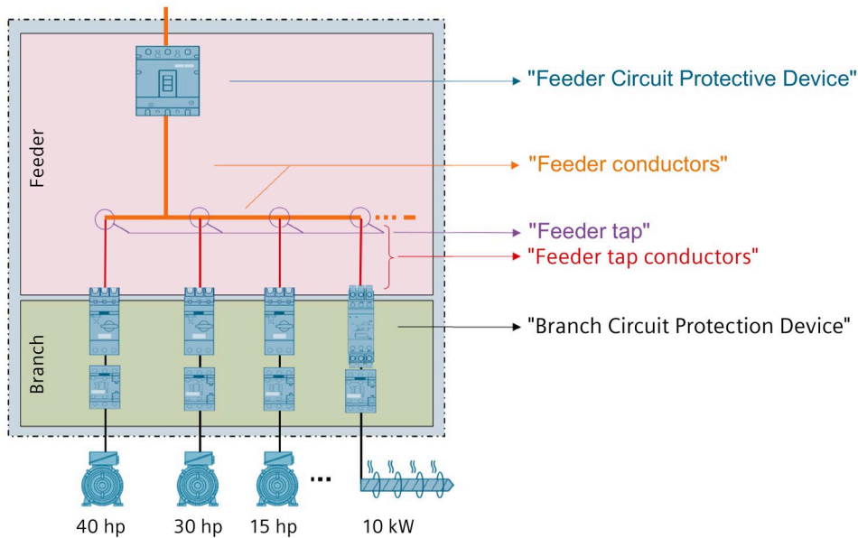
Figure 6-1 Overview of feeder and branch circuit of main circuits
