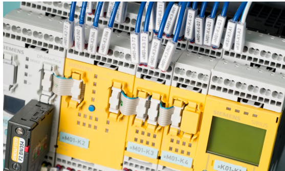
Figure 11-6 Example of conductor identification
