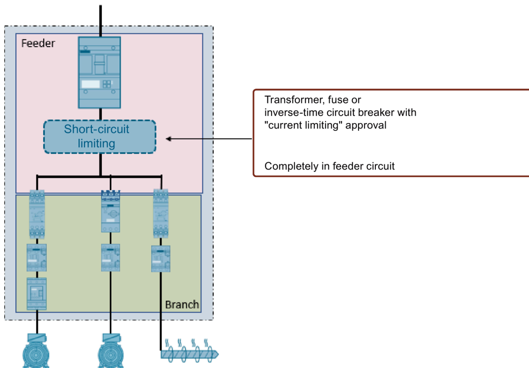
Figure 6-41 Diagram showing "short-circuit limiting in the feeder circuit"
