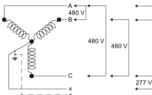
Figure 5-4 Line system configuration: Solidly grounded wye 480Y/277 V 3-phase, 4-wire
