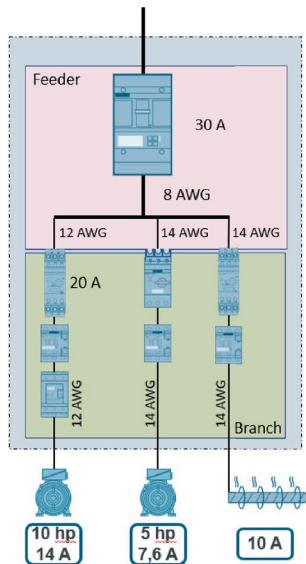
Figure 6-3 Result of the example for the dimensioning of the protection device in the Feeder Circuit
