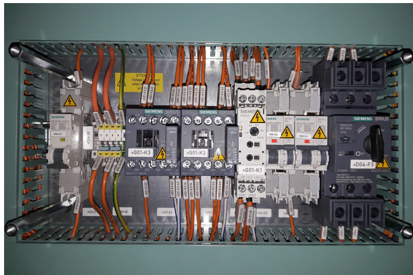
Figure 5-13 Example of the configuration of an excepted circuit
