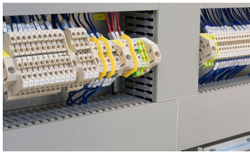
Figure 10-1 Grouping and separating terminals for the connection of external conductors
