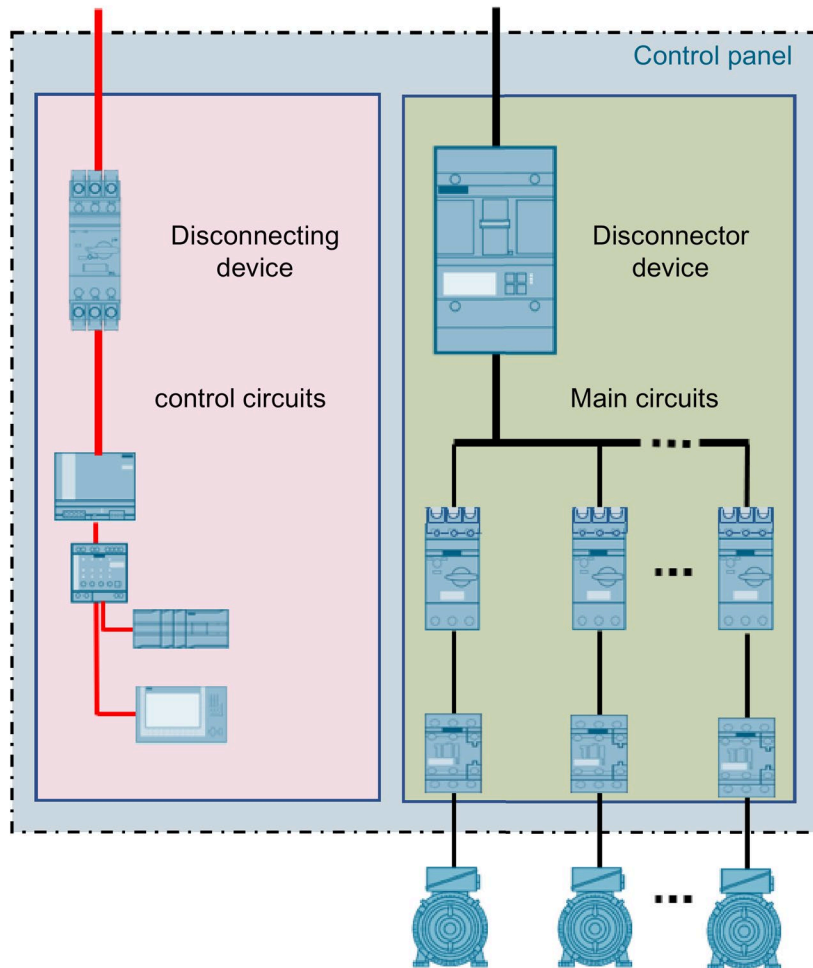
Figure 7-1 Control circuit with separate incoming supply circuit conductor
