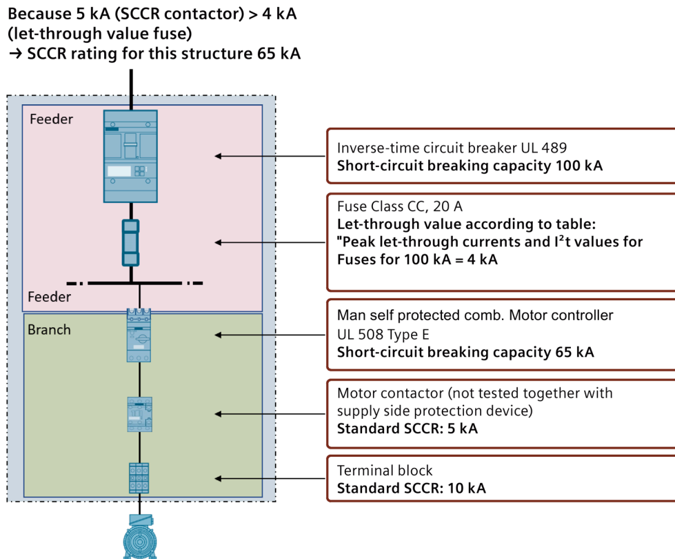
Figure 6-43 Example of "Determining the SCCR on the basis of a short-circuit-current-limiting fuse"
