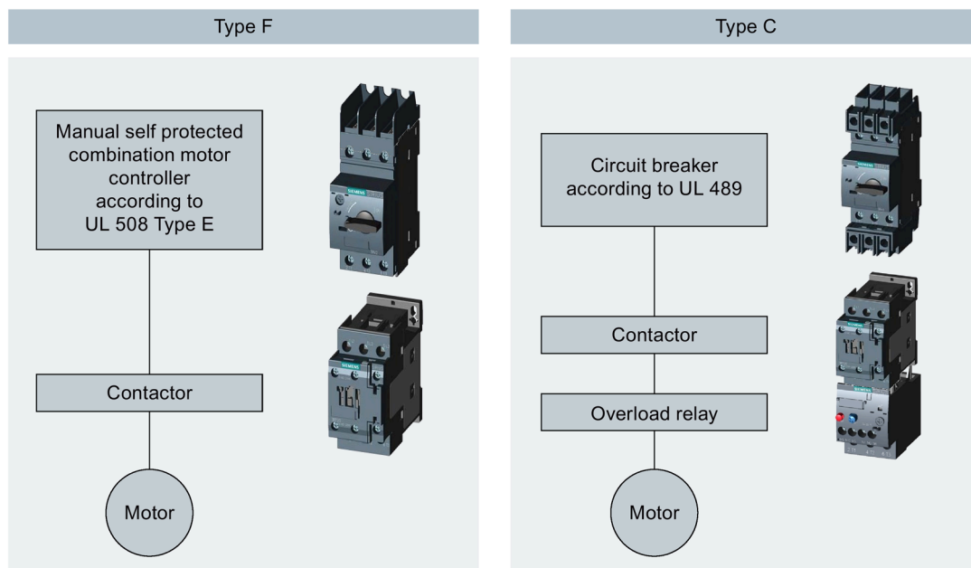
Figure 6-4 Examples of Type F and Type C
