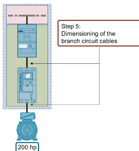
Figure 6-25 Sizing the cable
