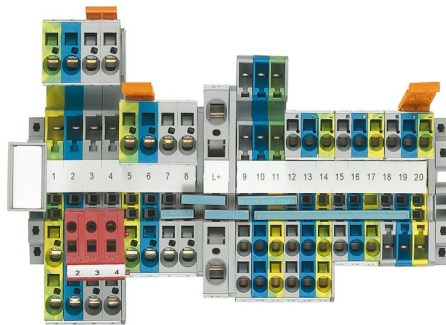
Figure 13-8 Siemens 8WH terminal arrangement
