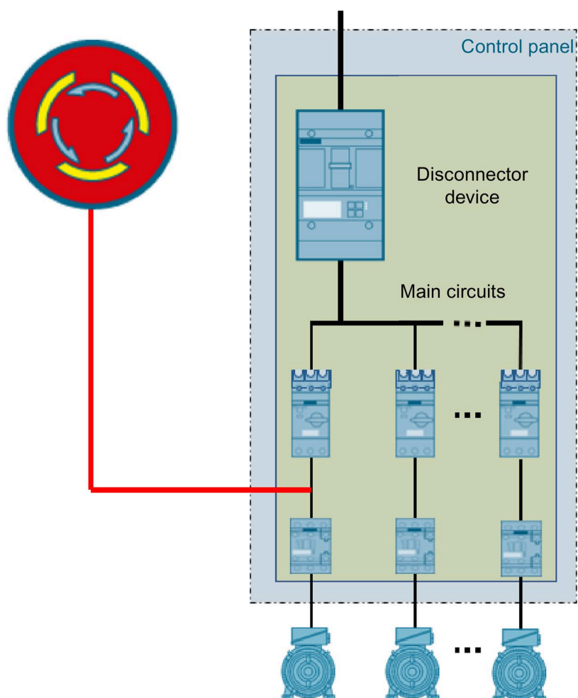
Figure 7-8 Tapping downstream of the main control switch downstream of the "Branch Circuit Protective Device" of a motor feeder without control circuit components outside the cabinet with remote control
